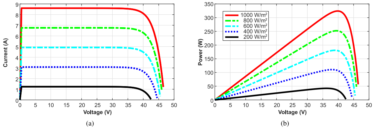
FIGURE 6. I-V and P-V characteristics for different irradiation values.
