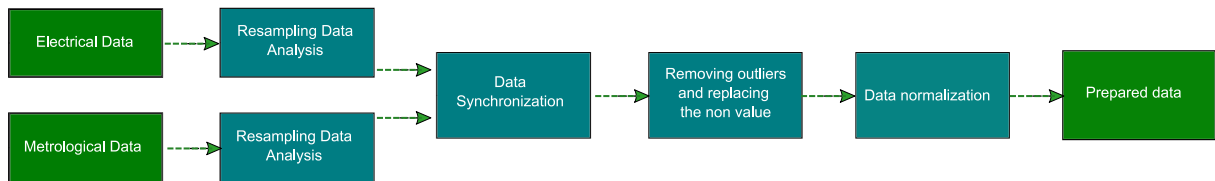
FIGURE 19. Data pre-processing stages.
